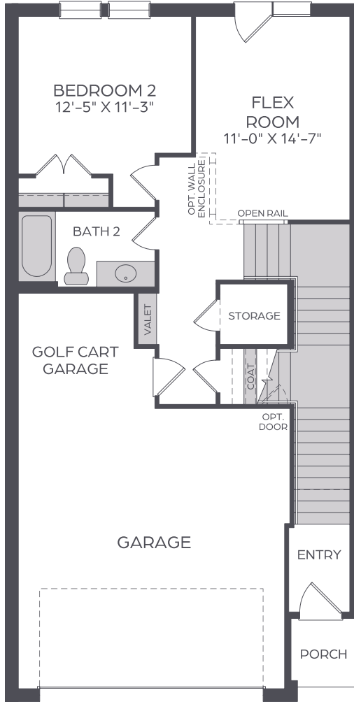
LOWER FLOOR
