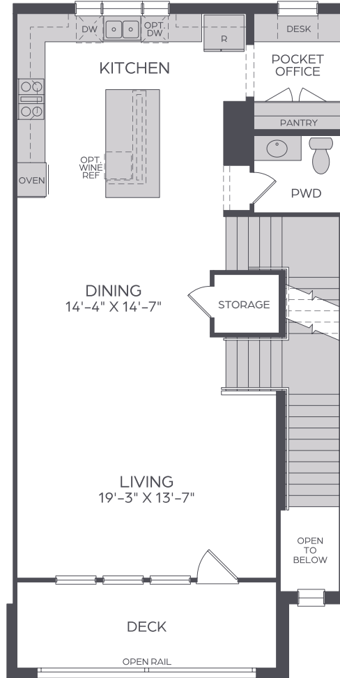
MAIN FLOOR
