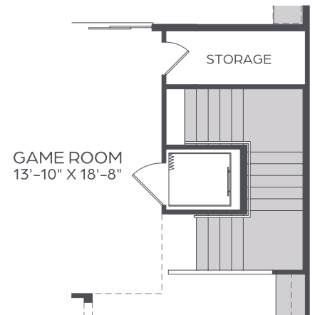
OPT. ELEVATOR
