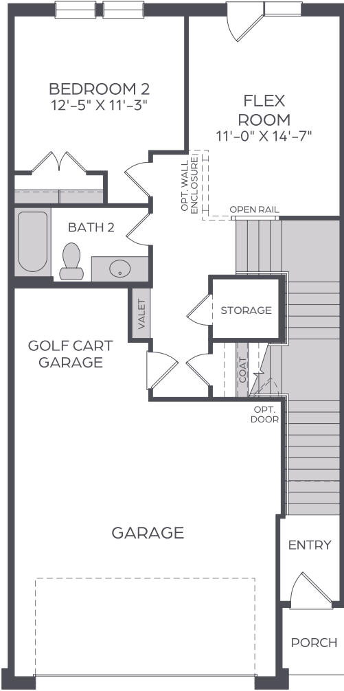
LOWER FLOOR
